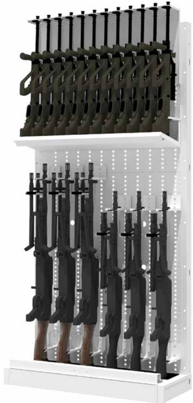
6 Mini-Mag or M1919 with 2 spare barrels on an EWR / 12 Steyr's on the top.
